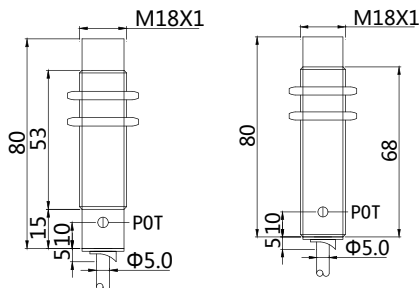
(Brass, nickel-plated)
