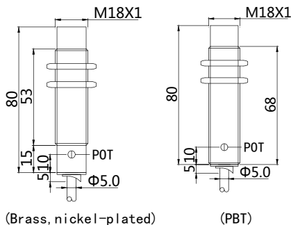
(Brass, nickel-plated)
